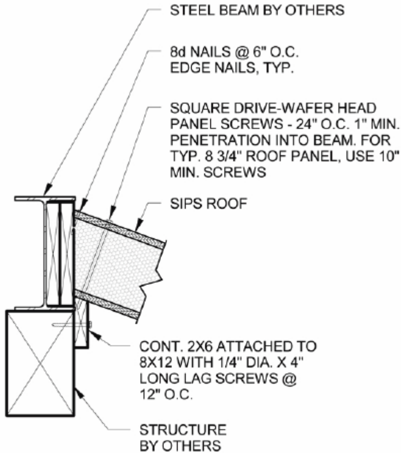
1 CONNECTION TO STEEL BEAM D9 1" = 1'-0"
