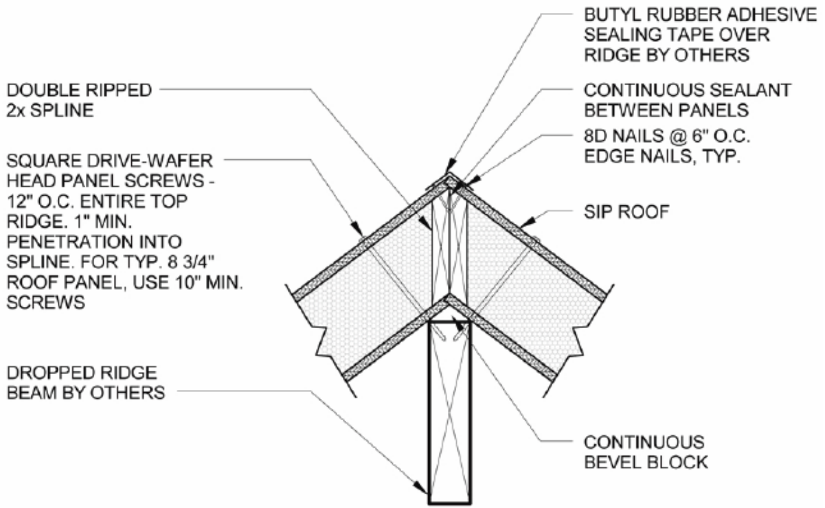
1 RIDGE BEAM @ ROOF DB 1" = 1'-0"
