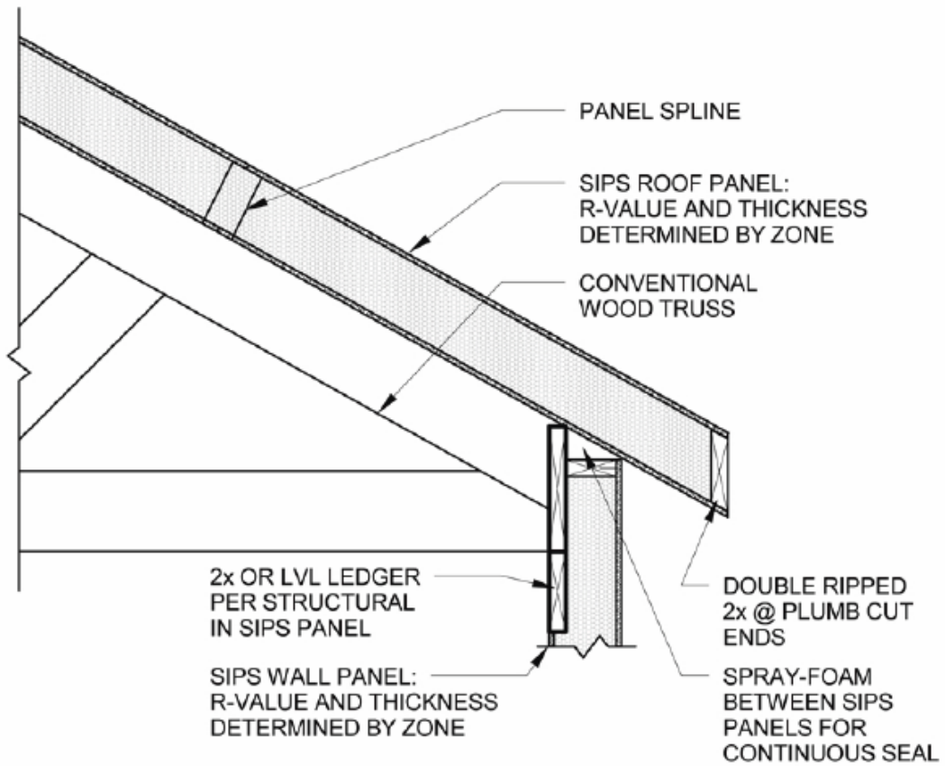
1 TRUSS W/ LEDGER D42 3/4" = 1'-0"
