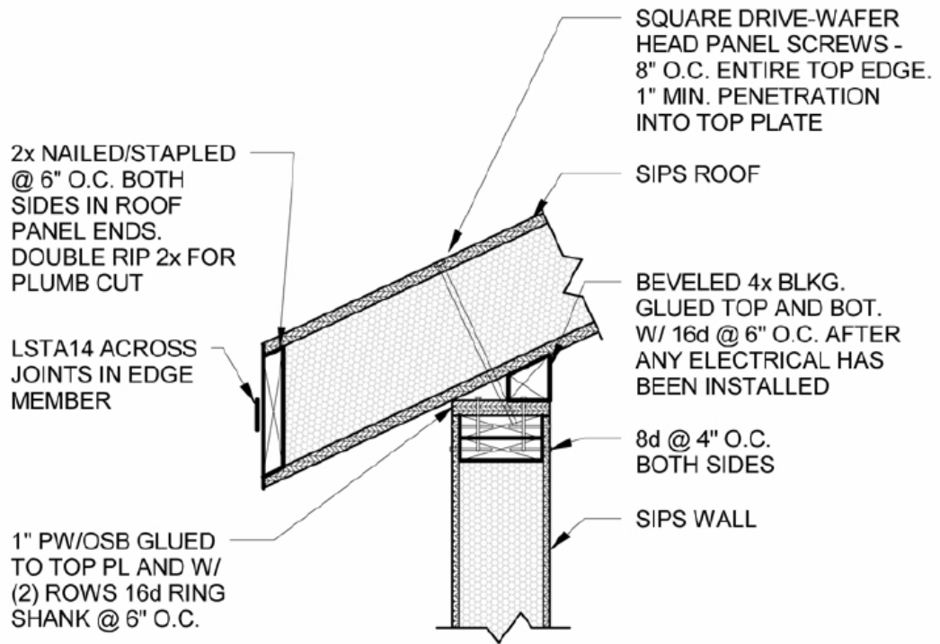
1 D4 ROOF EAVE TO WALL CONNECTION ALT. 1" = 1'-0"
