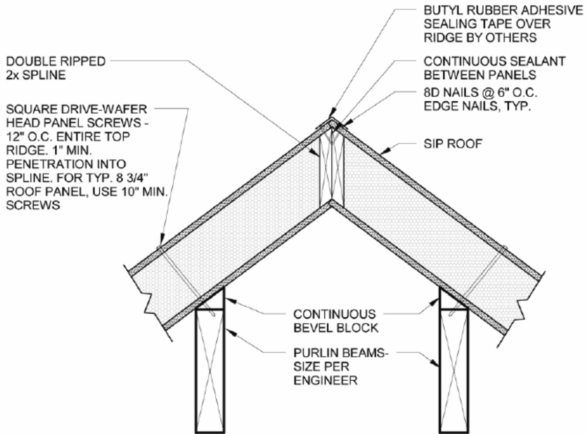
1 ROOF RIDGE W/ PURLINS D39 1" = 1'-0"
