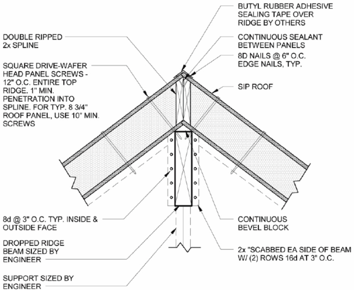
1 RIDGE BEAM @ END WALL 1" = 1'-0"
