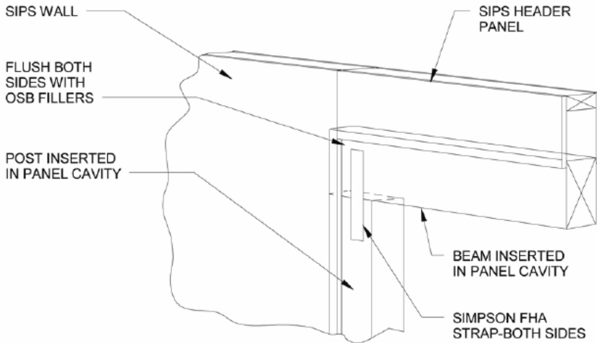
1 POST AND BEAM DETAIL D37 1/4" = 1'-0"
