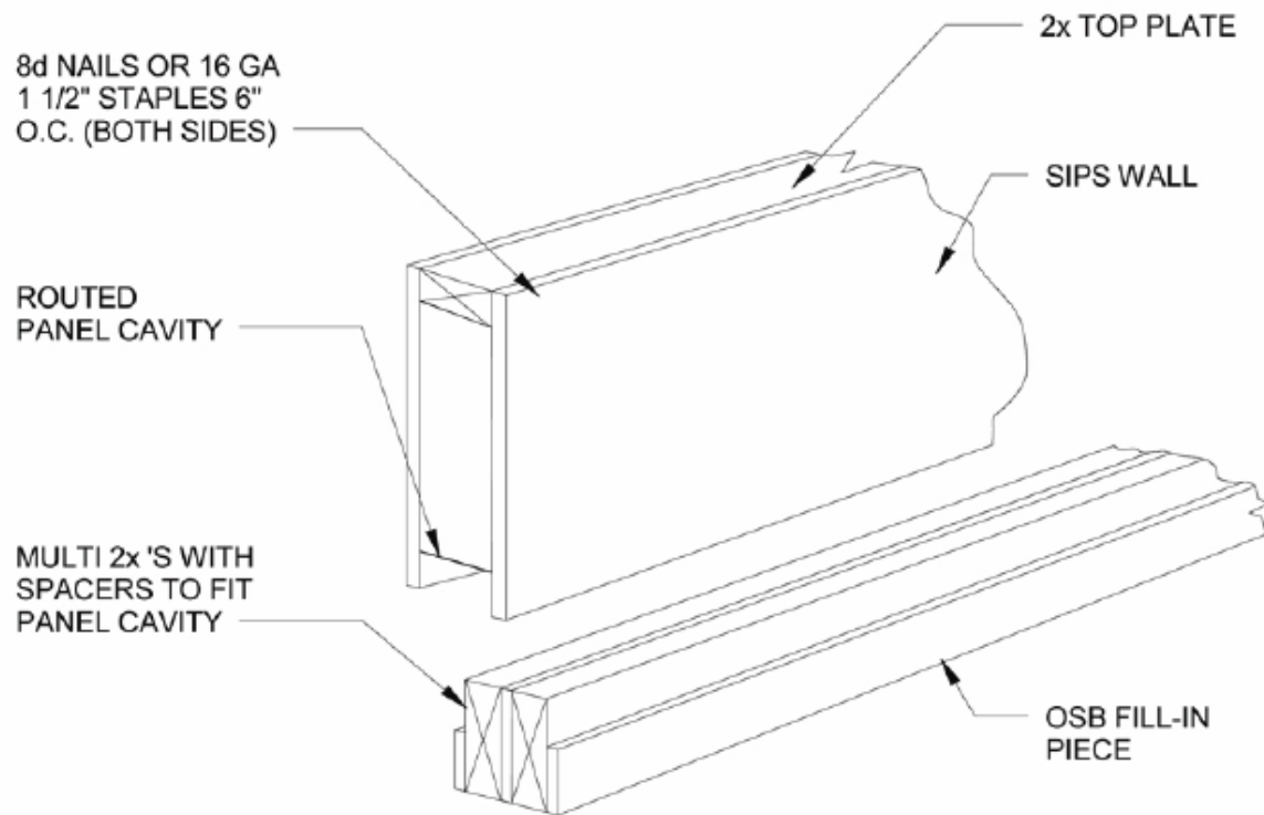
1 D33 BUILT-UP HEADER DETAIL 1/4" = 1'-0"
