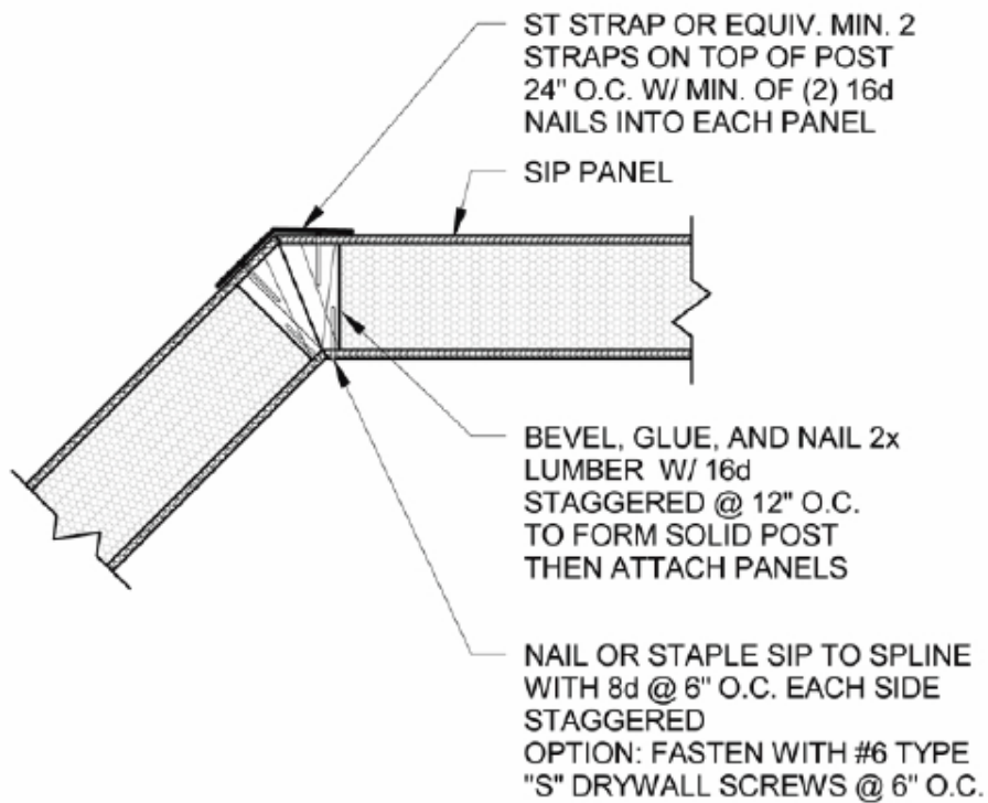
1 45 DEGREE POST DETAIL D31 1" = 1'-0"
