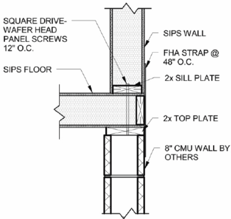
1 D30 2-STORY WALL/ SIPS FLOOR/CMU DETAIL 1" = 1'-0"
