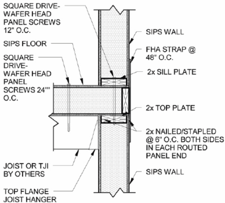
1 D28 2-STORY WALL/ SIPS/STRUCT FLOOR DETAIL 1" = 1'-0"
