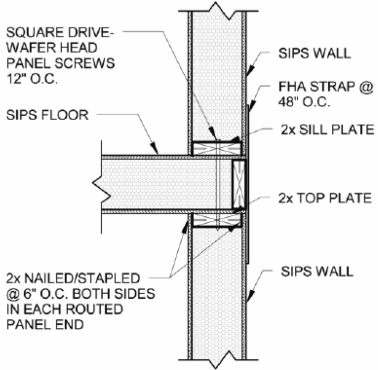
1 D27 2-STORY WALL/ SIPS FLOOR DETAIL 1" = 1'-0"
