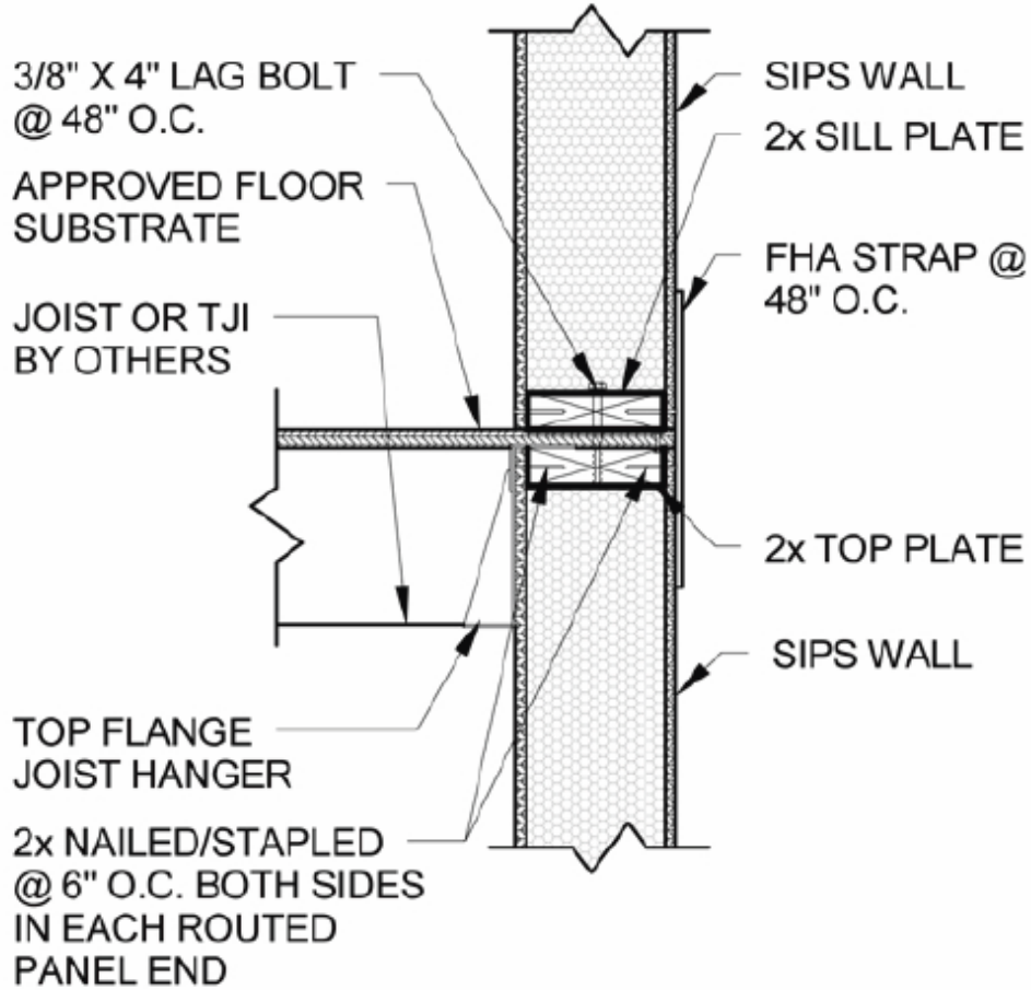
1 2-STORY WALL/FLOOR DETAIL D26 1" = 1'-0"
