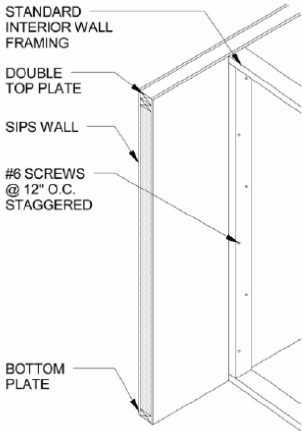
1 D22 INTERIOR WALL CONNECTION 1/2" = 1'-0"
