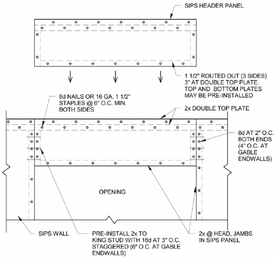
1 D21 DISCONTINUOUS PANEL HEADER 1" = 1'-0"
