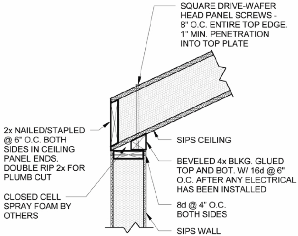
1 D2 WALL TO CEILING CONNECTION 1" = 1'-0"
