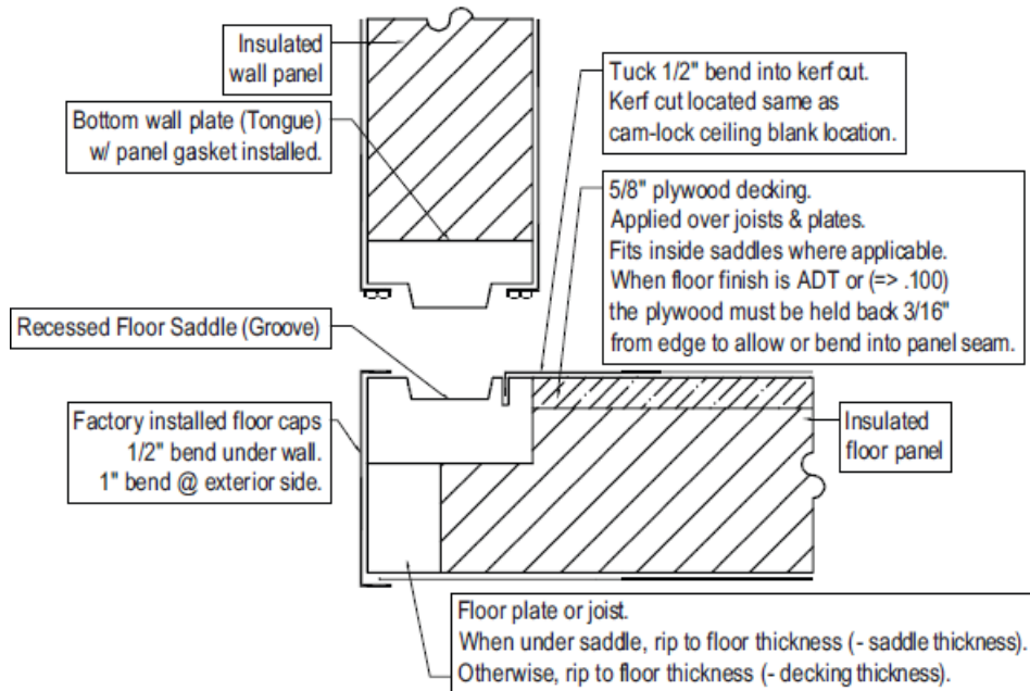
STANDARD FLOOR W/ RECESSED SADDLE
