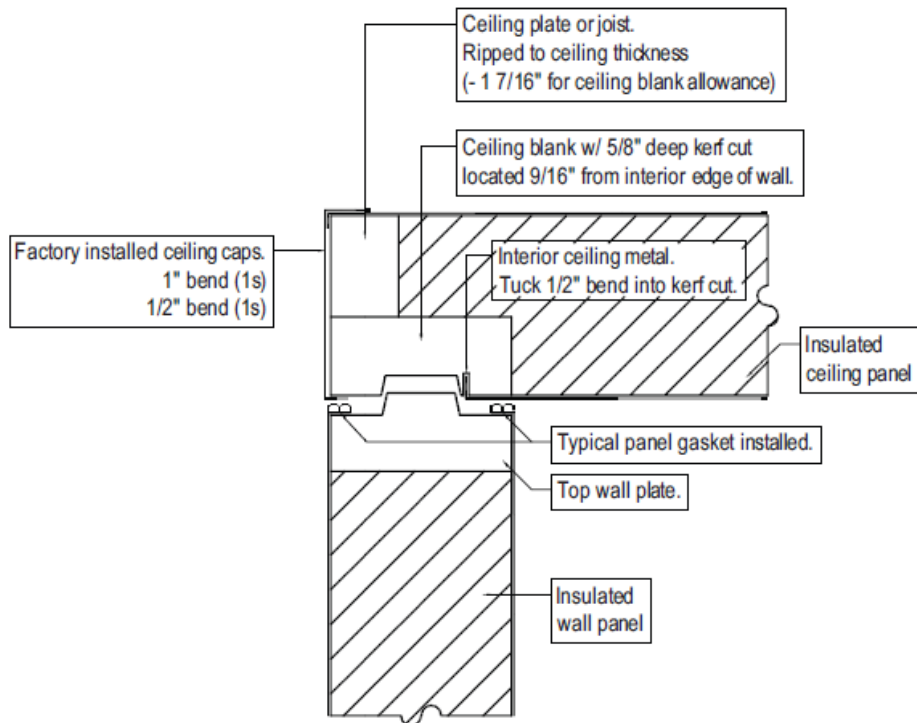
CAM-LOCK CEILING
